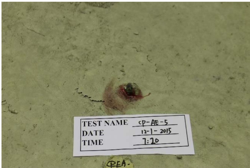
Figure B.32 Detailed view of the reinforcement at failure for CP-AE-5
