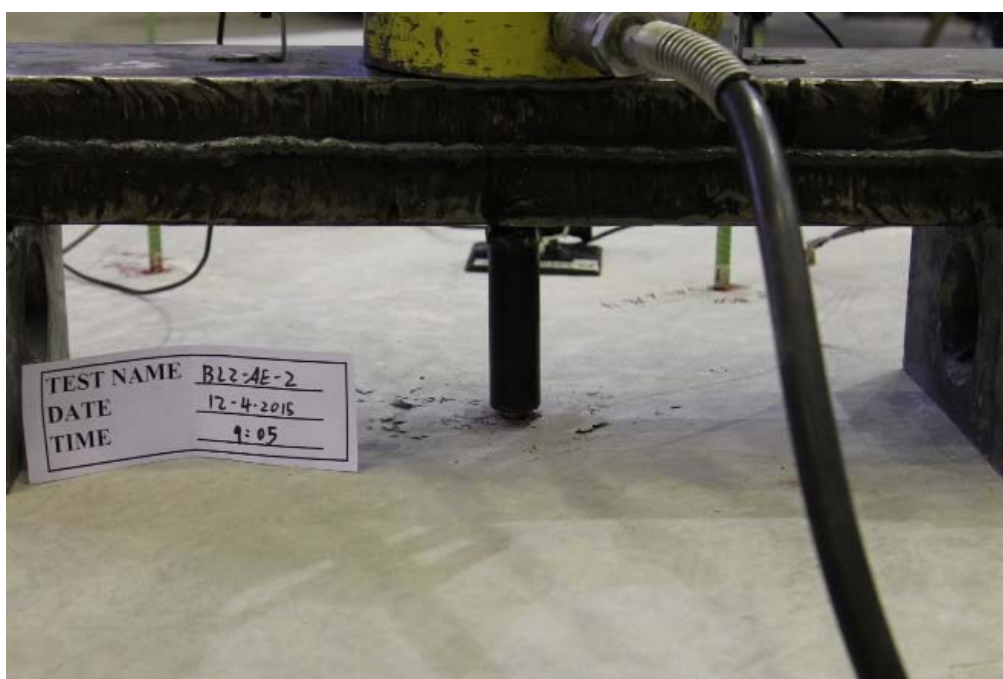
Figure B.5 Detailed view of the reinforcement at failure for BL-AE-2
